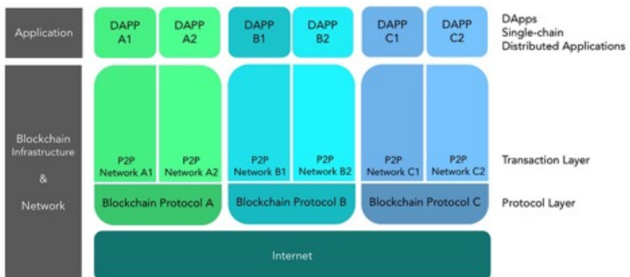
Figure 1: Representation of the current blockchain architecture.
